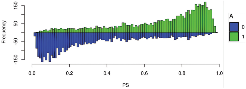
Figure 3. Distribution of the propensity score under the small overlap case.
