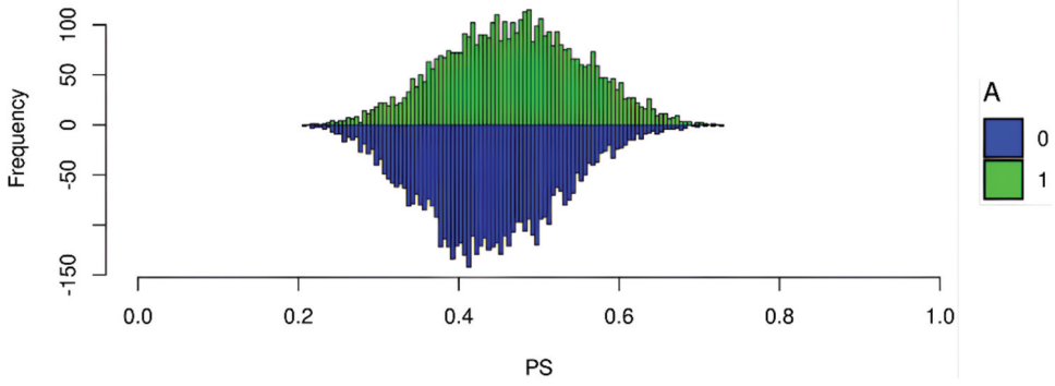
Figure 2. Distribution of the propensity score under the large overlap case.
