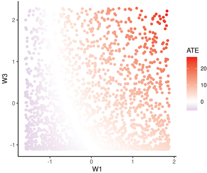
Figure 4. Treatment effect under heterogeneous treatment effect setting.
