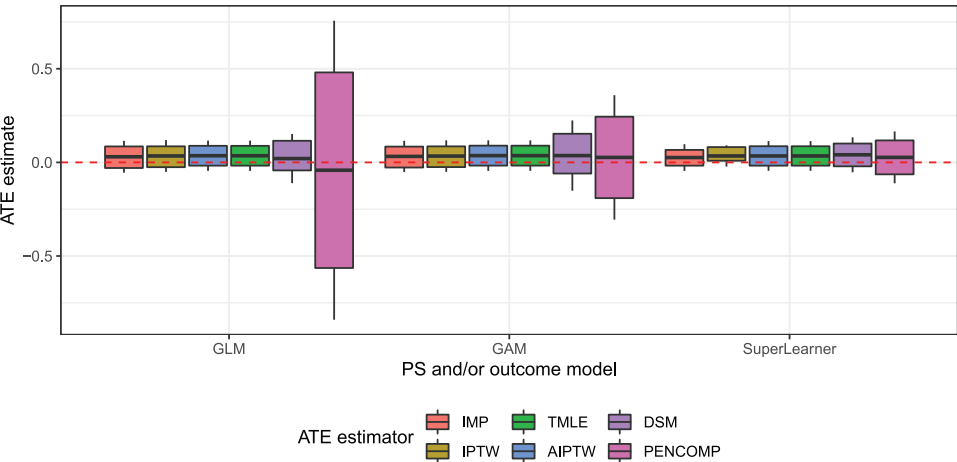
Figure 7. Performance of various causal estimators on the real-data application. Different colors imply different causal estimators, x-axis differentiate the PS and/or outcome models. The red dotted line indicates a zero ATE.
