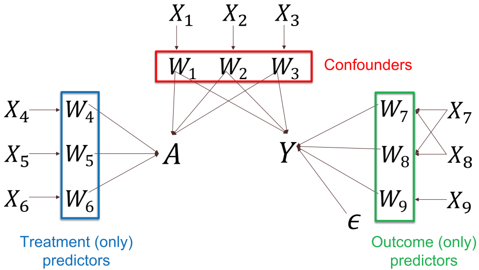
Figure 1. Illustration of variables involved in simulation studies.
